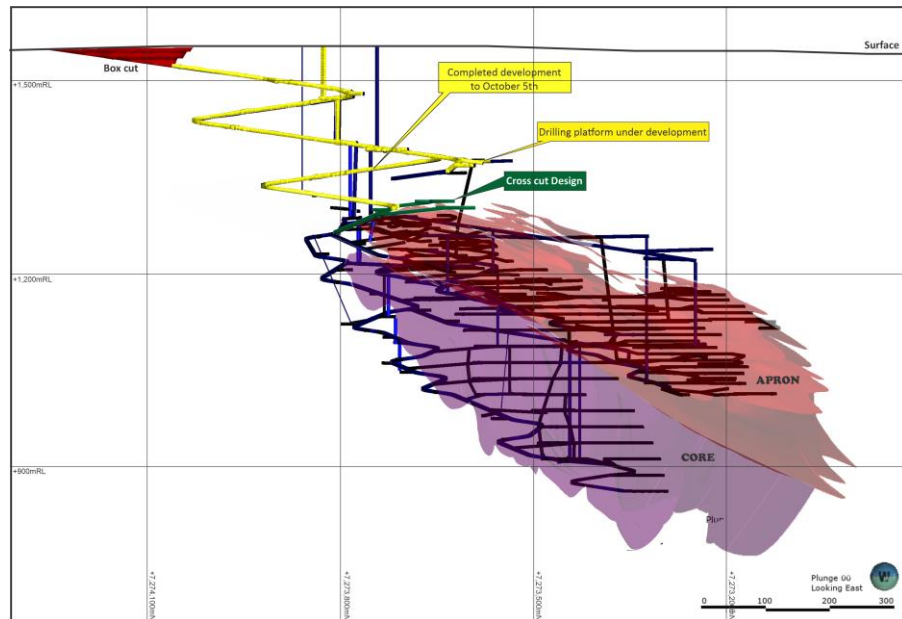
Abra Mine Schematic (September 2022)
